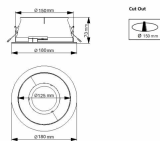
TCGSRR 150 20S/830 C PSU-E WH
